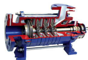
Model SRZS - Critical Process Specialty Pumps
